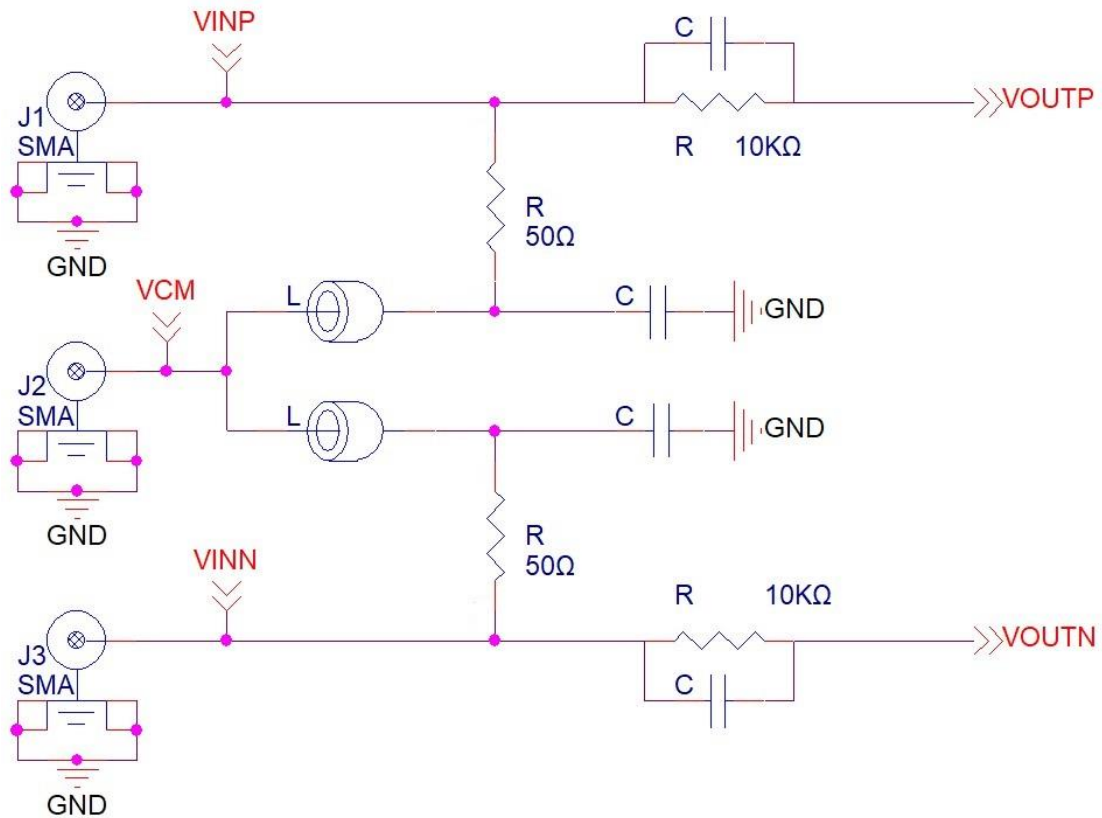
SMA-50 internal schematic diagram
