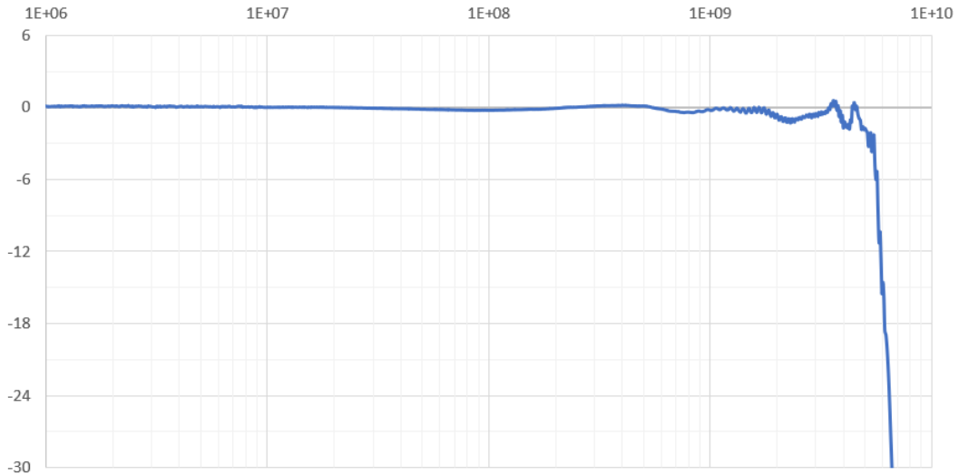
SSI-50 frequency response curve (welding 24.9R resistor)
