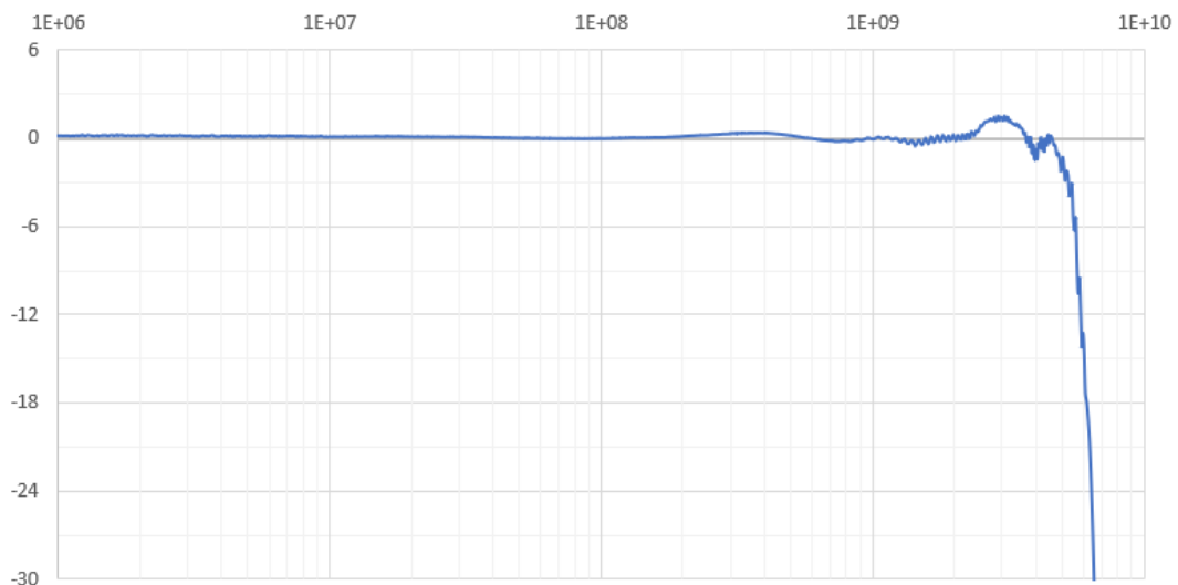
DSI-50 frequency response curve (welding 24.9R resistor)
