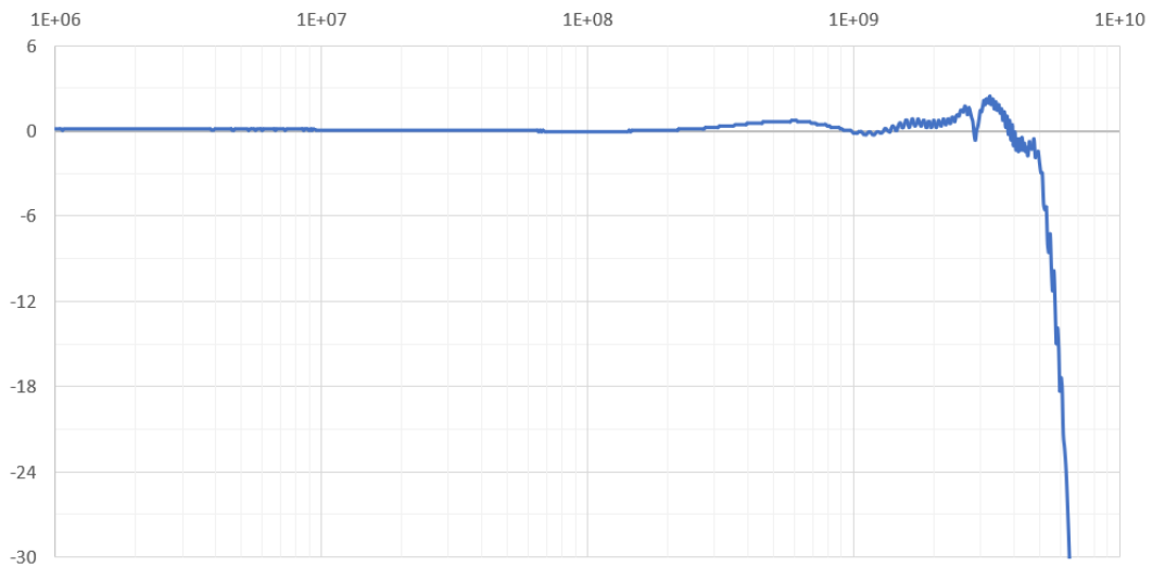
DBT-50 frequency response curve (with tungsten steel pin)
