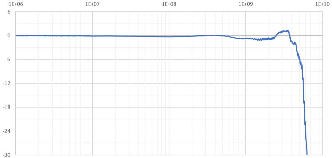
SRP-45 frequency response curve
