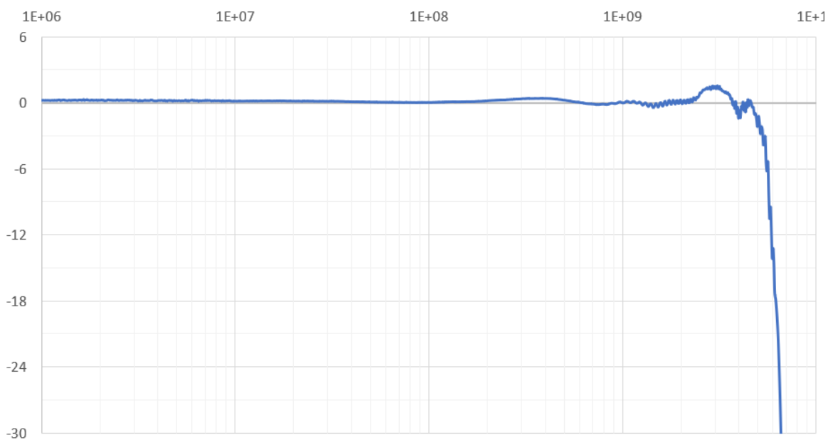
SAP5000D Frequency Response (DSI-50 Soldered 24.9Ω Lead Resistance)
