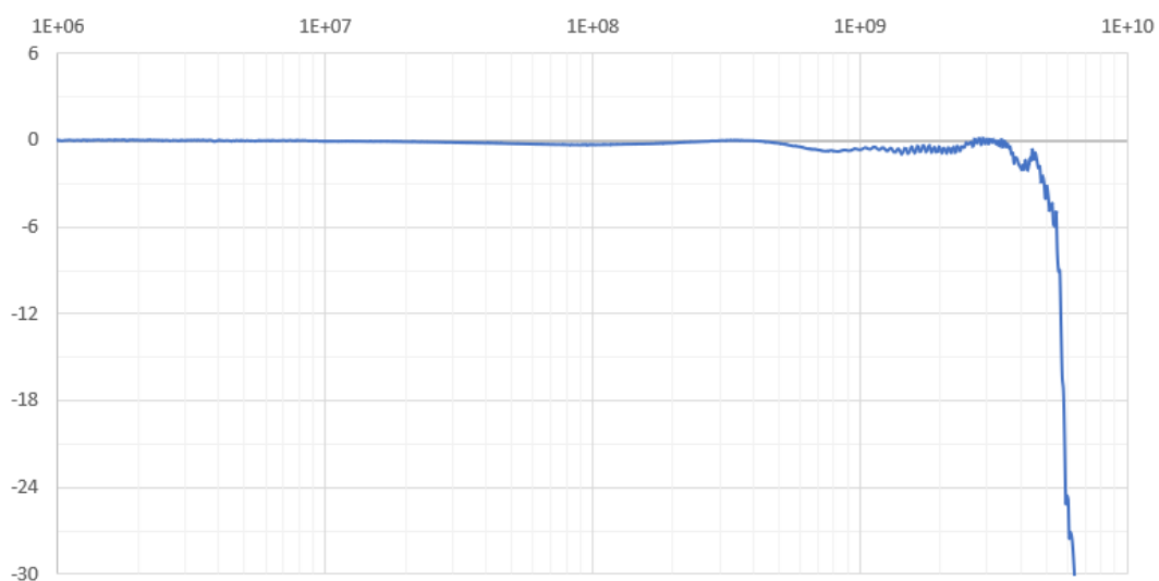
DRP-45 frequency response curve
