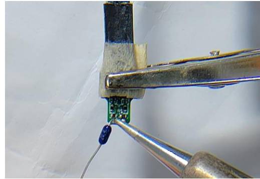
Lead Resistance Soldering
