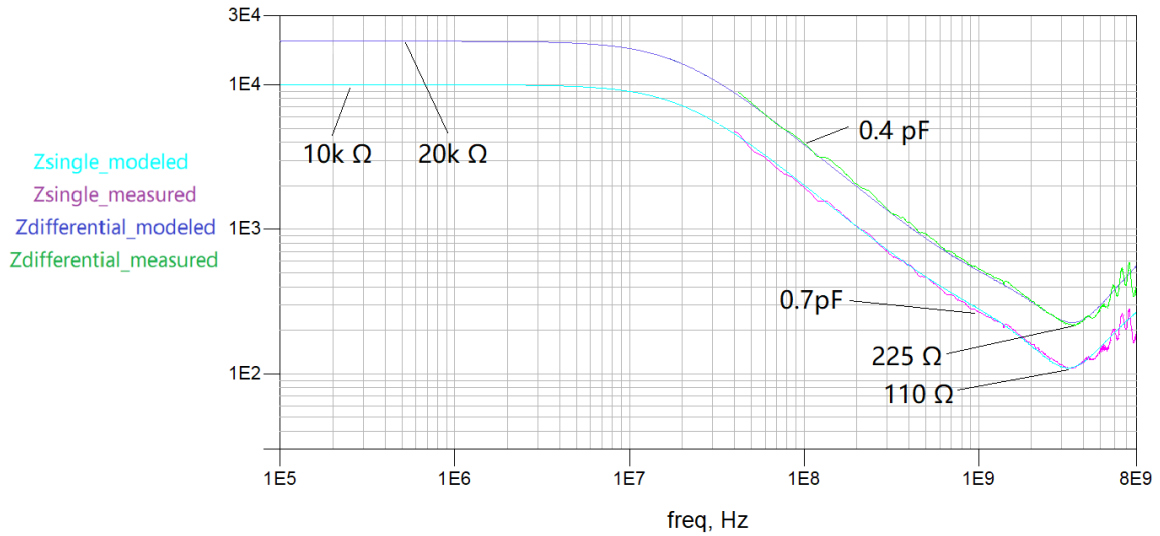
SAP5000D Input Impedance (DSI-50 Soldered 24.9Ω Lead Resistance)
