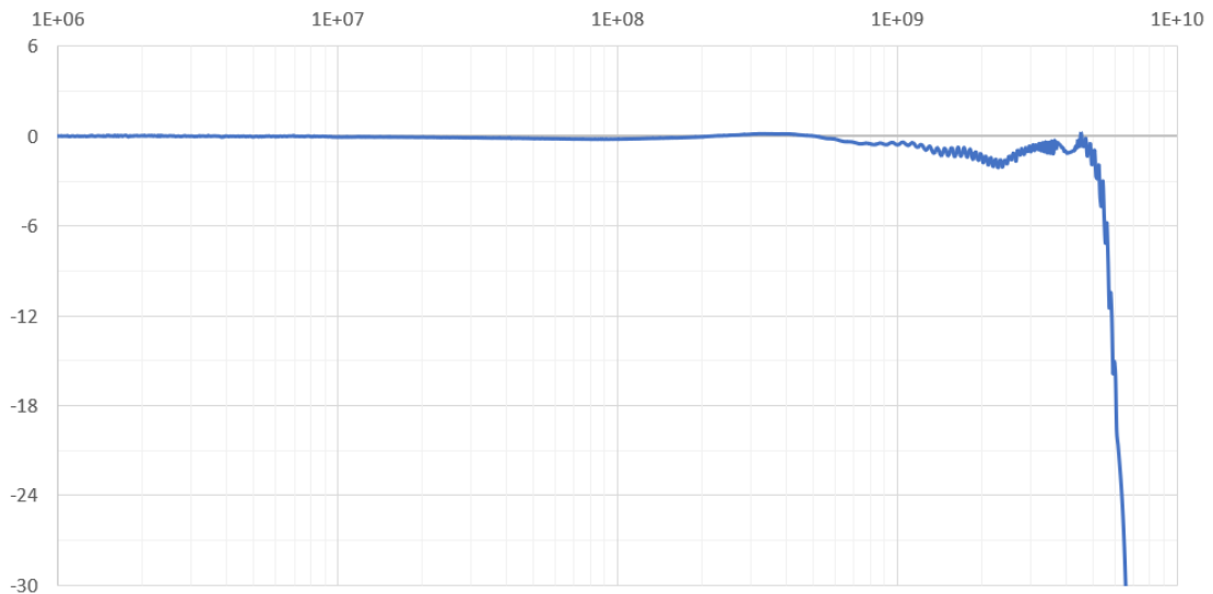
SMA-50 frequency response curve
